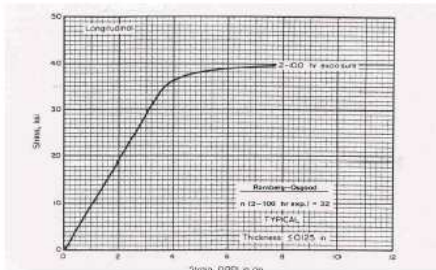
Figure 2. Tensile stress-strain curve of Aluminum alloy 6061-T6
